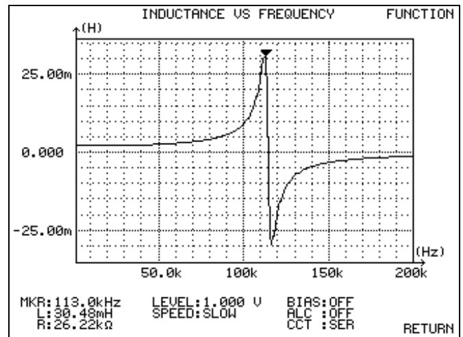
Inductance plotted against frequency
